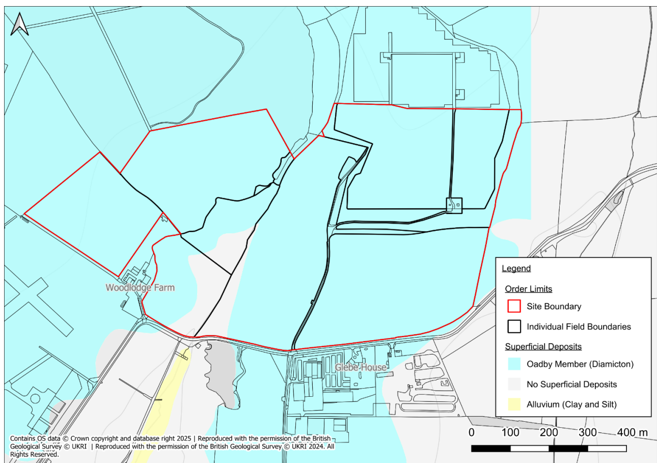
Figure 3: Superficial Deposits
